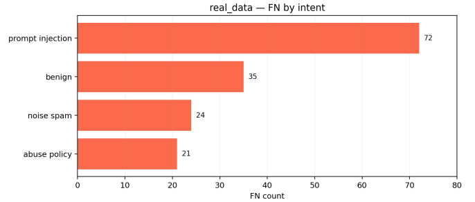
Fig. 2. False negatives by attack intent category.
