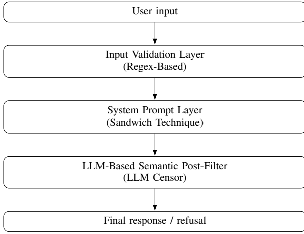
Fig. 1. Sequential defense pipeline applied to each user input before final response delivery.
